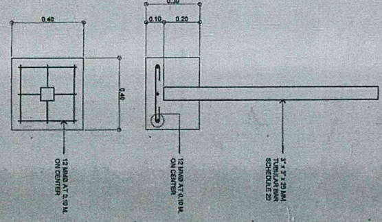
FOOTING DETAIL SCALE: 1:10M
